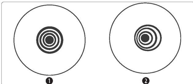
Figure 1. Correct (1) and incorrect (2) collimation as viewed during a star test.
